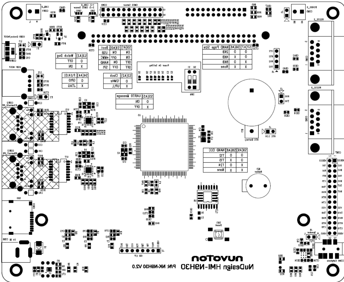
Figure 2-7 NuDesign NK-N9H30 Back PCB Placement
