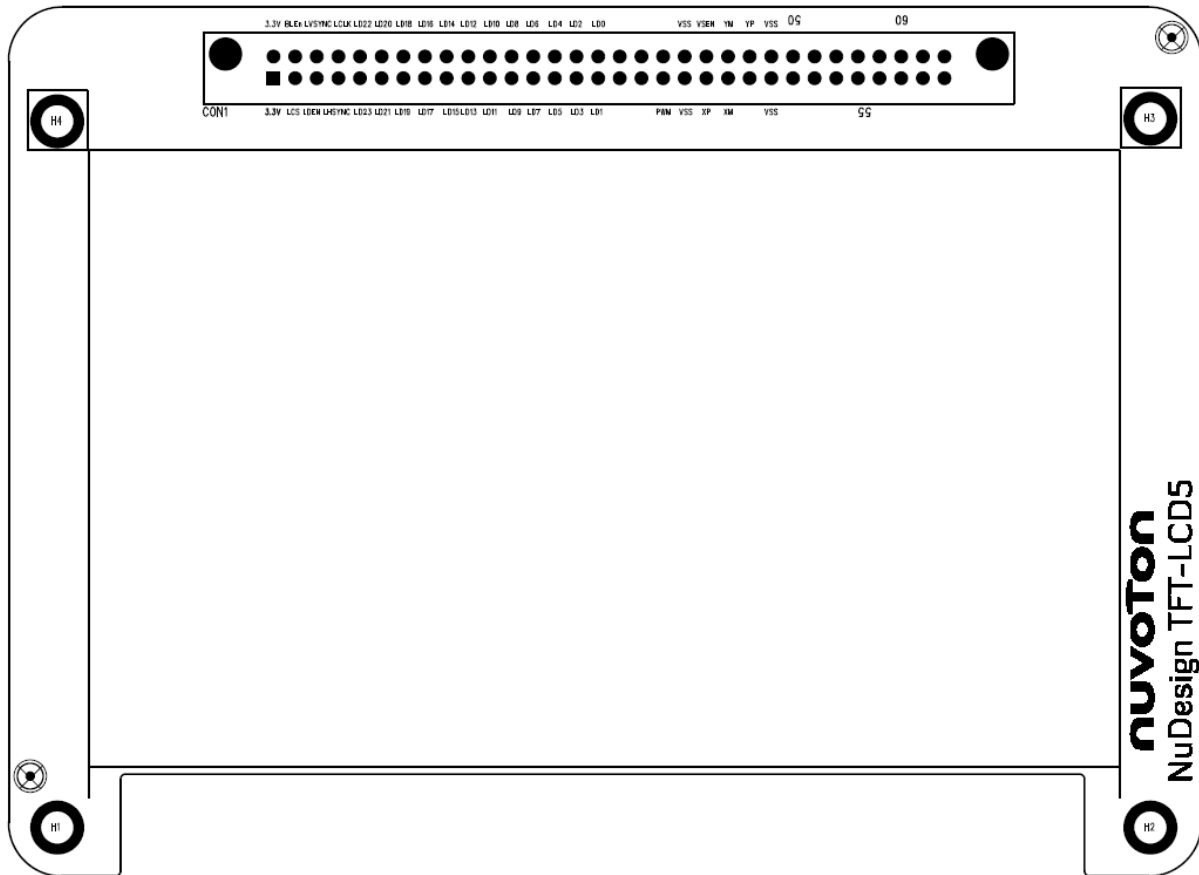
Figure 2-8 NuDesign TFT-LCD5 Front PCB Placement
