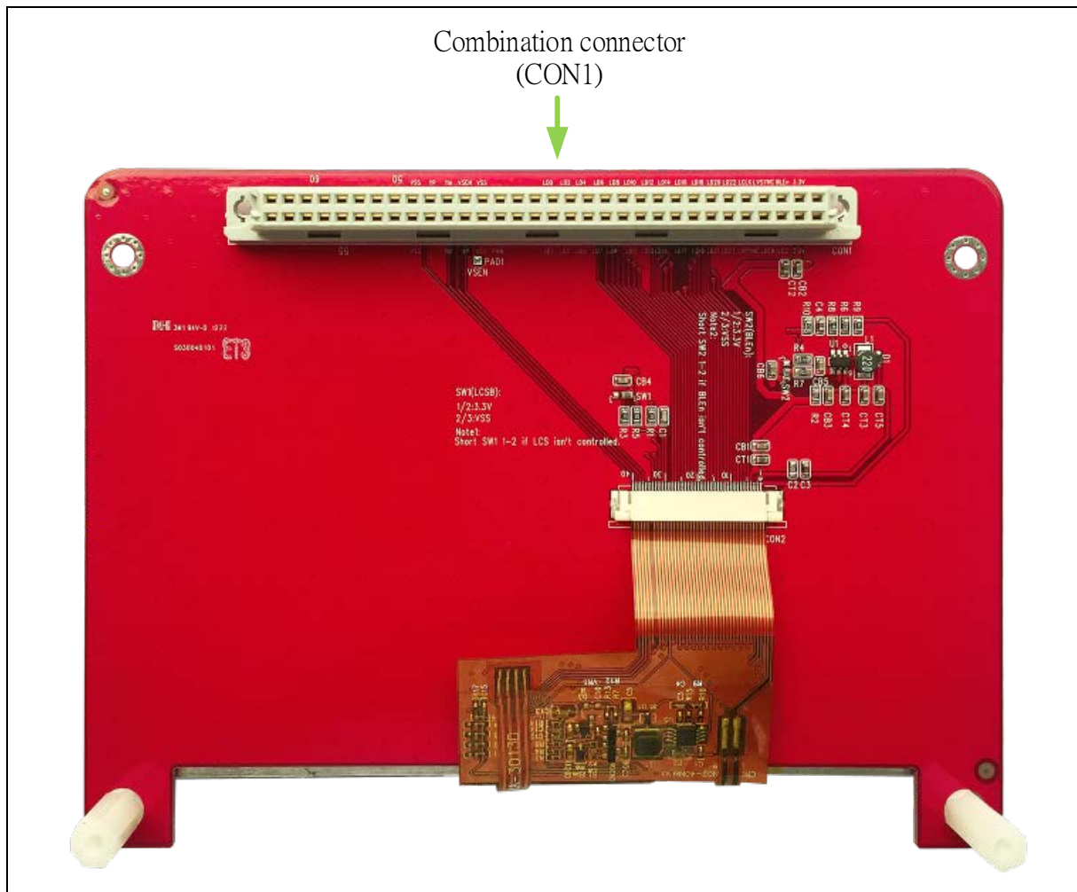
Figure 2-4 NuDesign TFT-LCD5 Board (Rear View)
