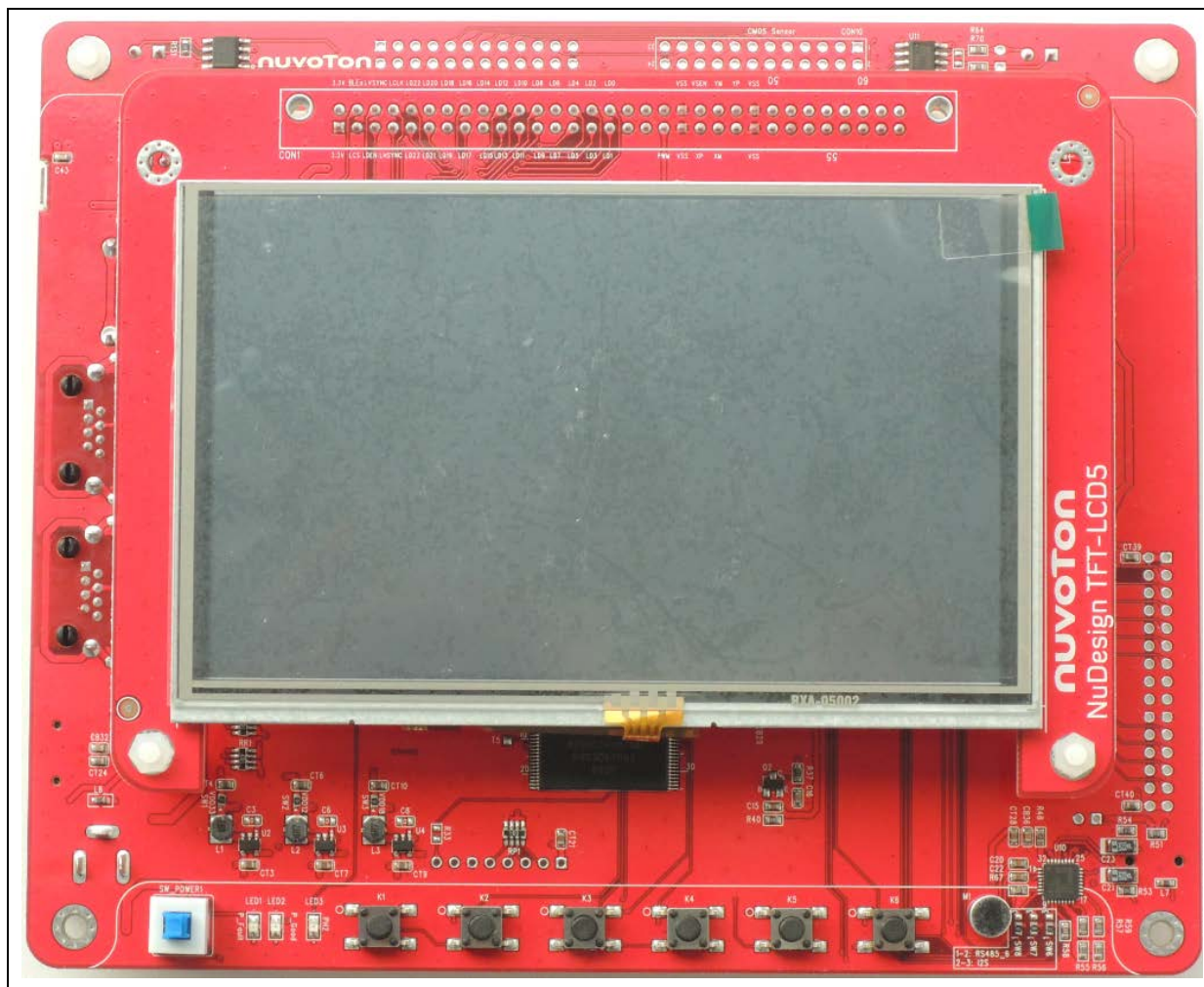
Figure 1-1 NuDesign NK-N9H30 Development Board (Front View)
