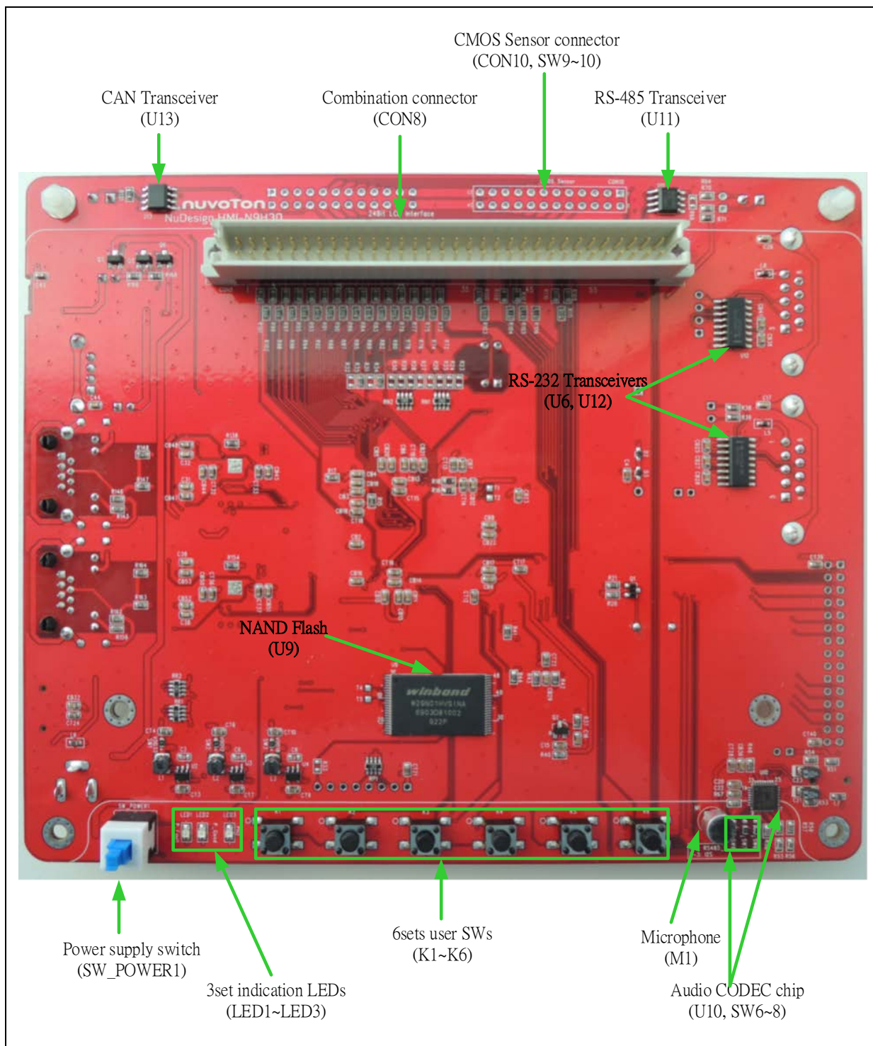
Figure 2-1 NuDesign NK-N9H30 Board (Front View)
