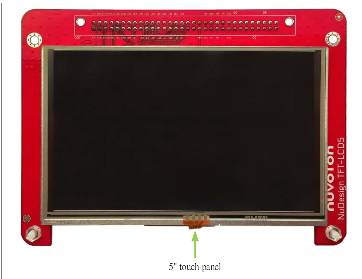
Figure 2-3 NuDesign TFT-LCD5 Board (Front View)
