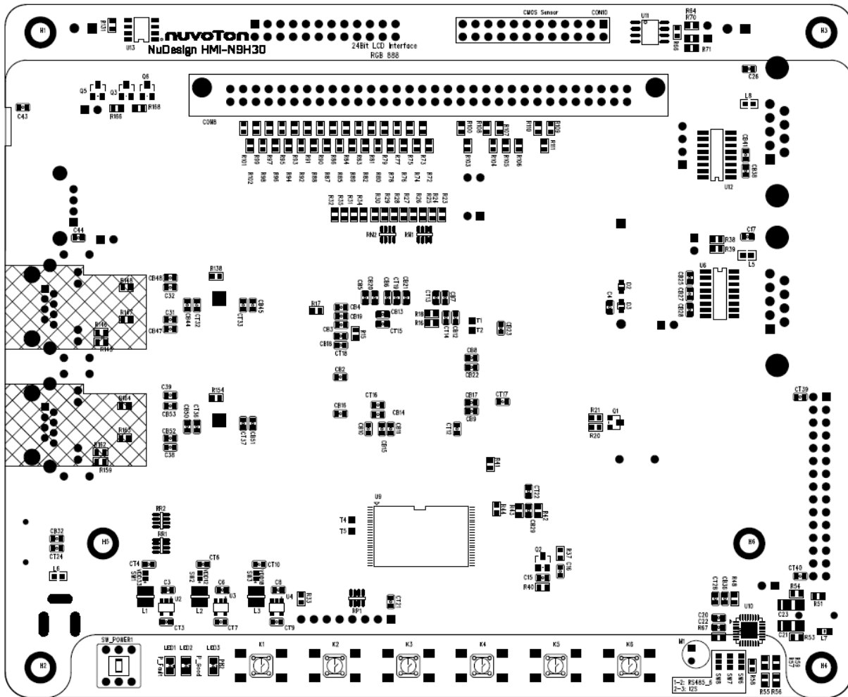
Figure 2-6 NuDesign NK-N9H30 Front PCB Placement
