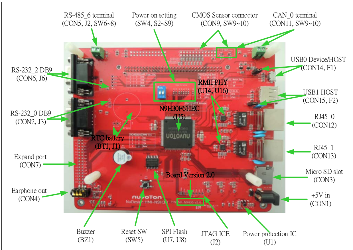
Figure 2-2 NuDesign NK-N9H30 Board (Rear View)
