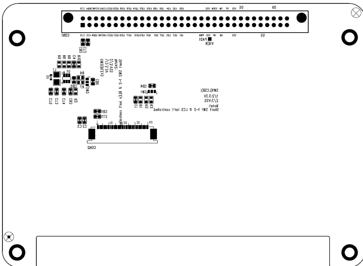
Figure 2-9 NuDesign TFT-LCD5 Back PCB Placement
